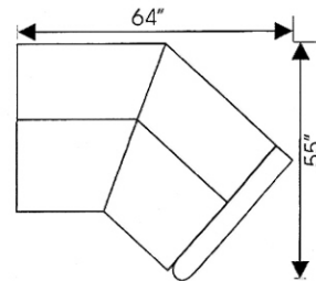
797-47 RF ANGLE LOVESEAT 68W 38D 33H
